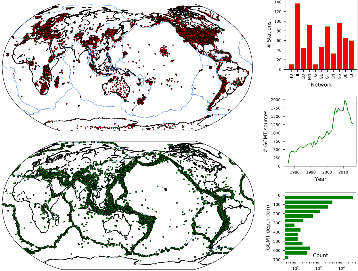
Figure 1. Global map showing the reported locations of 44 871 sources (green hexagons) recorded on 12 222 receivers (red inverted triangles) that contributed to the analysis. All locations with at least a single associated measurement from the eight contributing groups (Table 1) are included. Bar graph shows the number of stations (out of 10 469) from a few representative networks (out of 310) available from the open IRIS data centre. Also shown are the yearly count and depth distribution of the 40 122 earthquakes between 1976 and 2016 validated against the Global CMT catalogue (Section 4.4). Plate boundaries (Bird et al. 2009) are shown in light blue.
