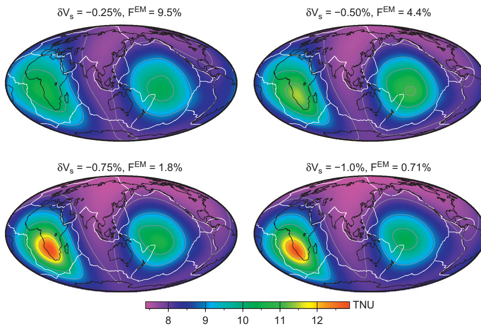
Fig. 3. Global map of geoneutrino event rate in TNU from 238 U + 232 Th decay in the mantle calculated for the TOMO model using geochemical BSE and A&McD DM compositional estimates, and several different cut-off \delta V_s contours (indicated above each map together with the resulting mass fraction of the enriched mantle reservoir F^{EM} ). A unique radius for the crust–mantle boundary is used (6346.6 km), flux is evaluated at radius of 6371 km and shown in TNU with contour lines at 1 TNU intervals. Continental outlines (black) and plate boundaries (white) are plotted. Color scale is identical for all four maps. (For interpretation of the references to color in this figure caption, the reader is referred to the web version of this article.)
