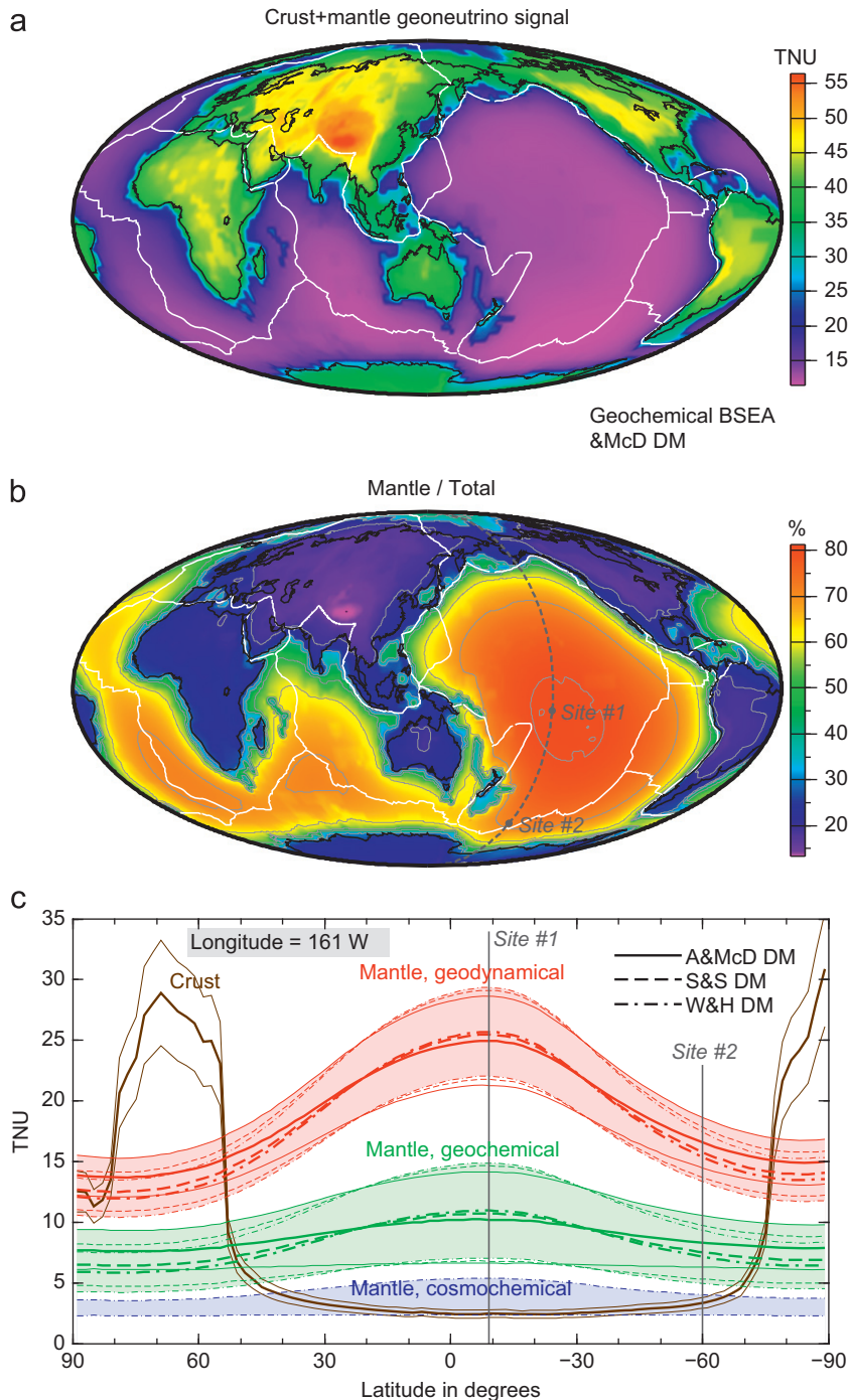
Fig. 4. (a) Global map of predicted total geoneutrino signal ( ^{238}\text{U} + ^{232}\text{Th} , crust+mantle) in TNU. Mantle anti-neutrino emission model same as in Fig. 2. Crustal prediction based on CRUST2.0 structure, and R&G, W&K and Plank compositional estimates (see text). Topography of the crust–mantle boundary is accounted for geoneutrino fluxes are evaluated at zero elevation in oceanic areas and at Earth’s surface in continental regions. Continental outlines (black) and plate boundaries (white) are shown. (b) Map showing the fraction of total signal from panel “a” that is contributed by the mantle; the remainder is the crustal contribution. Contour lines at 10% intervals. (c) Variation of predicted geoneutrino signal along 161°W meridian which intersects the Pacific mantle flux maximum at 9°S. Crustal prediction shown in brown. Mantle predictions based on cosmochemical, geochemical, and geodynamical BSE estimates shown in blue, green, and red, respectively. Central values (thick curves) and 1\sigma uncertainty limits (thin lines and shading) are shown. Two oceanic measurement sites are proposed (shown in panels “b” and “c”) in order to constrain Earth’s mantle architecture. (For interpretation of the references to color in this figure caption, the reader is referred to the web version of this article.)
