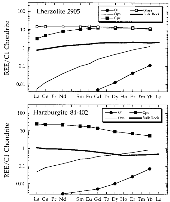
Fig. 3. REE diagram for bulk-rock peridotites and their minerals for sample 2905, a LREE-depleted, fertile lherzolite and 84-402 and a LREE-enriched, harzburgite. REE abundances are normalized to C1 chondrites using the values reported in McDonough and Sun [28]. REE abundances in the spinels are at or below detection limits. Ol = olivine; Opx = orthopyroxene; Cpx = clinopyroxene; Amph = amphibole breakdown glass.
