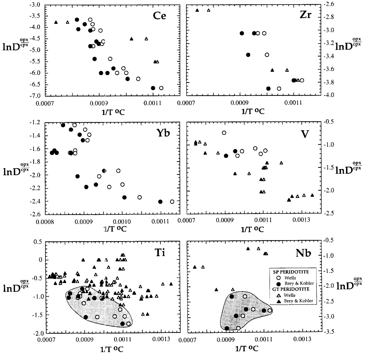
Fig. 8. 1/T ( ^{\circ}\text{C} ) vs. \ln D^{\text{opx/cpx}} for Ce, Yb, Ti, Zr, V and Nb in spinel- (circles) and garnet-facies peridotites (triangles). Temperatures are derived from two calibrations of the two-pyroxene thermometer [17,18], thus two points are plotted for each sample (in some cases the two temperatures coincide). REE partitioning data are from both bulk mineral [20,35,39] and in situ methods (this study and [40]). Ti data are either by electron microprobe studies in which attention was paid to obtaining high-quality analyses [10,41,42] or from LA-ICP-MS (this study). V data from electron microprobe [41,42] or LA-ICP-MS (this study). Zr and Nb data are from ion microprobe [40], solution ICP-MS [35,39] and LA-ICP-MS (this study). Data for peridotites with multiple generations of minerals were omitted (e.g., [11,43]).
