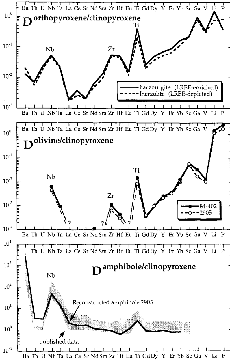
Fig. 7. Mineral/mineral partition coefficients for co-existing phases in the herzholite (2905) and harzburgite (84-402). Many of the olivine data for the highly incompatible elements are at the level of detection limits. Bottom panel shows amphibole/clinopyroxene partitioning from this study (reconstructed amphibole from sample 2905, see Appendix A) compared to field of published results [11,21,35–38]. In addition to our study, Th and U partitioning data are only available from Chazot et al. [21] and Ionov and Hofmann [35]. Ol = olivine; Opx = orthopyroxene; Cpx = clinopyroxene; Glass = amphibole breakdown glass.
