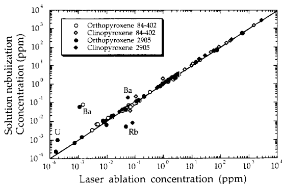
Fig. 2. Comparison of trace-element abundances in clinopyroxene and orthopyroxene from 2905 as determined by solution nebulization ICP-MS and laser ablation ICP-MS. Element abundances are given in ppm ( \mu\text{g}/\text{g} ). Anomalies in Ba and U are likely due to impurities in the mineral separates, whereas the anomalies in Rb are due to high background during laser ablation analyses (see text).
