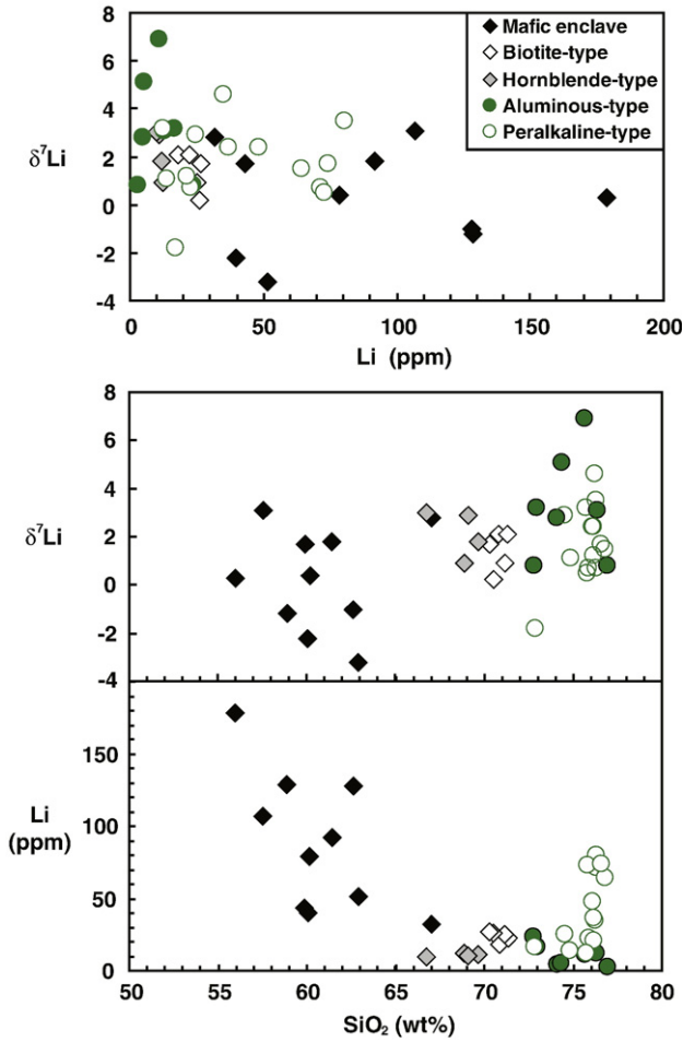
Fig. 3. Plots of Li and \delta^7\text{Li} vs. \text{SiO}_2 for A-type granites and mafic enclaves. Data are from Tables 1 and 2 and references cited therein.
