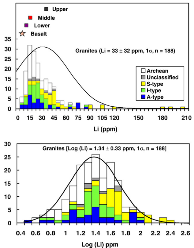
Fig. 9. Upper panel: Li concentrations of 188 worldwide post-Archean A-type, I-type and S-type granites, as well as unclassified granites and Archean TTG gneisses (see data compilation provided in the on-line supplement). The distribution of Li concentration in these granites is skewed to higher values, yielding an arithmetic average Li of 33 \pm 32 ppm ( 1\sigma ). The average Li concentration of the upper, middle and lower continental crust, as well as fresh oceanic basalts are plotted for comparison. Lower panel: distributions of Log(Li) concentrations of the same population as in the upper panel. The data form a normal distribution with an arithmetic average Log(Li) of 1.34 \pm 0.33 ppm ( 1\sigma ), corresponding to a geometric average Li concentration of 22 ppm, a lower limit of 10 ppm and the upper limit of 47 ppm. The normal distribution curves calculated from the means and standard deviations are shown. Data sources are the same as for Fig. 8 except Archean TTG gneiss, which are from Mohan et al. (2008) and Teng et al. (2008).
