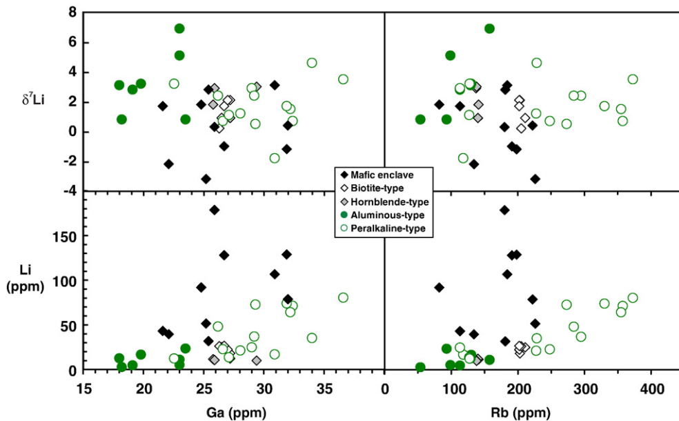
Fig. 4. Plots of Li and \delta^7\text{Li} vs. Ga and Rb for A-type granites and mafic enclaves. Data are from Tables 1 and 2 and references cited therein.
