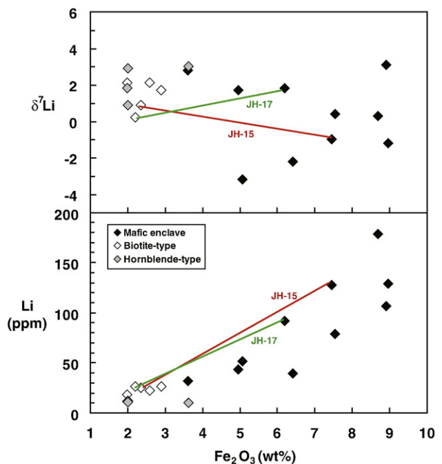
Fig. 6. Plots of Li and \delta^7\text{Li} vs. \text{Fe}_2\text{O}_3 for mafic enclaves and A-type granites from the Qianshan pluton, North China craton. Tie-lines show the mafic enclaves JH-15-2 and JH-17-2 and their adjacent host granites JH-15-1 and JH-17-1 respectively. Data are from Table 2 and references cited therein.
