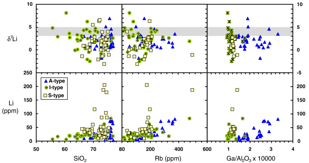
Fig. 7. Plot of Li concentrations and isotopic compositions vs. SiO 2 , Rb and Ga/Al 2 O 3 × 10,000 for worldwide post-Archean A-, I- and S-type granites (see data compilation provided in the on-line supplement). A-type granite data are from Tables 1 and 2; I-type granite data are from Bryant et al. (2004), Teng et al. (2004) and Marks et al. (2007); S-type granite data are from Teng et al. (2004, 2006b) and Bryant et al. (2004). The gray bar represents the Li isotopic compositions of fresh oceanic basalts (Ryan and Langmuir, 1987; Chan et al., 1992; Chan and Frey, 2003; Ryan and Kyle, 2004; Elliott et al., 2006; Tomascak et al., 2008; Schuessler et al., 2009).
