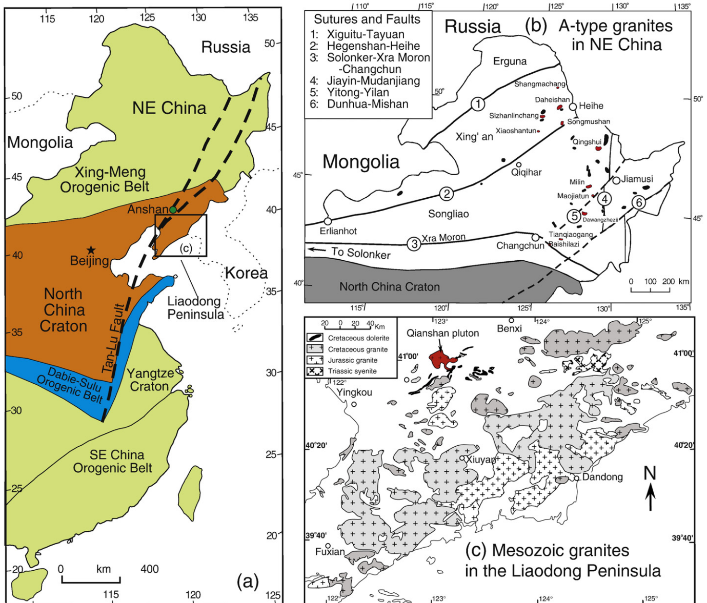
Fig. 1. Simplified geologic map of eastern China showing sample locations. The major tectonic divisions are also plotted. Modified from Wu et al. (2002) and Yang et al. (2006).
