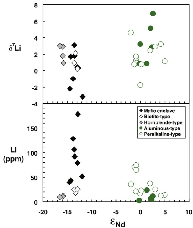
Fig. 5. Plots of Li and \delta^7\text{Li} vs. \epsilon_{\text{Nd}} for A-type granites and mafic enclaves. Data are from Tables 1 and 2 and references cited therein.
