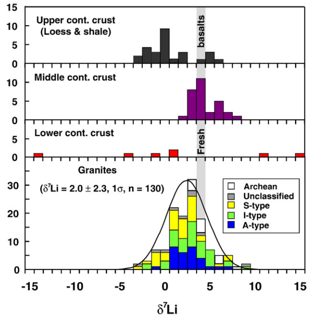
Fig. 8. Lithium isotopic compositions of 130 worldwide post-Archean A-type, I-type and S-type granites, as well as unclassified granites and Archean TTG gneisses (See data compilation provided in the on-line supplement). The data form a normal distribution, with a weighted average δ 7 Li of +1.7 and an arithmetic mean of +2.0 ± 2.3 (1σ). The normal distribution curve calculated from the arithmetic mean and standard deviation is also shown. The Li isotopic compositions of the upper (Teng et al., 2004), middle (Teng et al., 2008) and lower (Teng et al., 2008) continental crust, as well as fresh oceanic basalts, are plotted for comparison. Data sources for post-Archean A-, I- and S-type granites, as well as fresh oceanic basalts, are the same as for Fig. 7. Unclassified granite data are from James and Palmer (2000), Pistiner and Henderson (2003), Rudnick et al. (2004), Teng et al. (2004) and Tomascak et al. (2003). Archean TTG gneiss data are from Teng et al. (2008).
