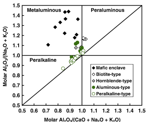
Fig. 2. Plots of molar Al 2 O 3 /(Na 2 O + K 2 O) vs. Al 2 O 3 /(CaO + Na 2 O + K 2 O) for A-type granites and mafic enclaves. Data are from Wu et al. (2002) and Yang et al. (2006).
