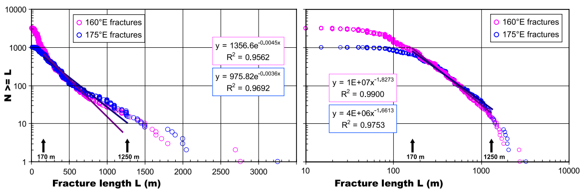
Figure 22. Cumulative frequency ( N = number) plot of ~N160°E (in pink) and ~N175°E (in blue), 170- to 1250-m-long fracture lengths ( L ). (left) Log linear scale with exponential fit for both populations. (right) Log-log scale plot with power law fit for both populations. The power law fit is generally the best, with an exponent of 1.83 and 1.66 for ~N160°E and ~N175°E fractures.
