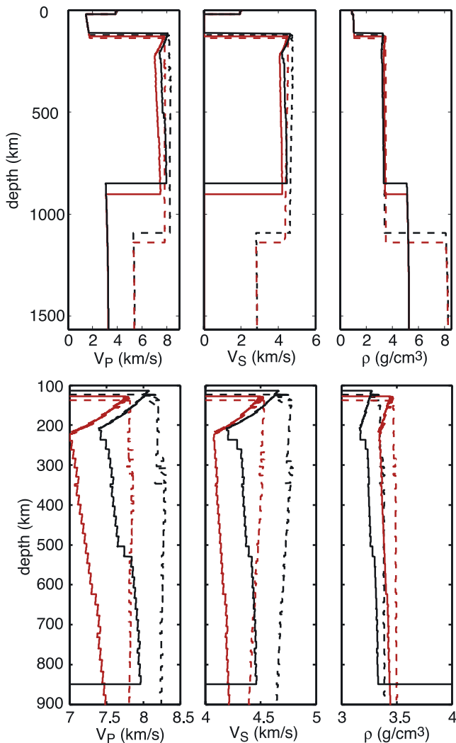
Figure 6. Physically consistent models for hot (solid lines) and cold (dashed) thermal structures for pyrolitic mantle (black) or chondritic (red). The bottom panel shows a mantle close-up of the same models.
