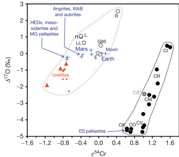
Figure 1 A plot of \Delta^{17}\text{O} (deviation from the terrestrial fractionation line in a \delta^{17}\text{O} vs. \delta^{18}\text{O} plot, in ‰) plotted against \epsilon^{54}\text{Cr} (deviation from terrestrial ^{54}\text{Cr}/^{52}\text{Cr} in parts per ten thousand) demonstrates the isotopic nonuniformity of solar system materials. A similar variability is seen for the neutron-rich isotopes of titanium and nickel. Carbonaceous chondrites are clearly separated from other chondrite types and the planets. The difference between main group (MG) and Eagle Station (ES) pallasites seems to indicate two different parent bodies for pallasites. The figure is taken from Warren PH (2011) Stable-isotopic anomalies and the accretionary assemblage of the Earth and Mars: A subordinate role for carbonaceous chondrites. Earth and Planetary Science Letters 311: 93–100.
