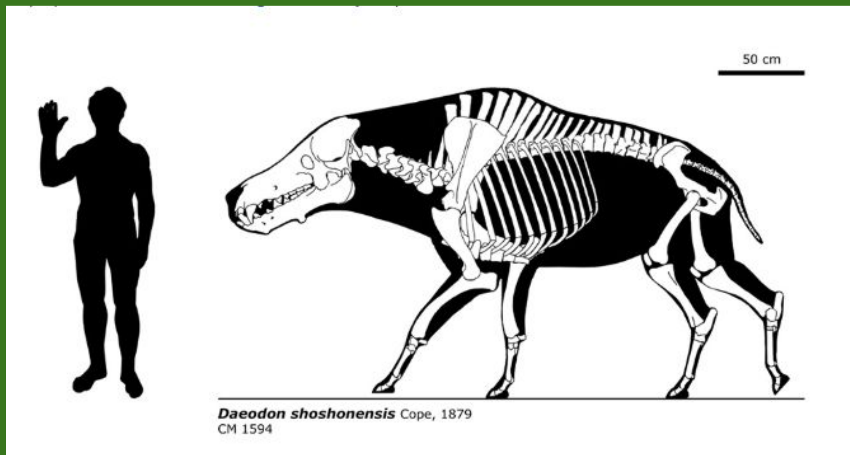
A. Illustrative of the skeleton of the Entelodont and human comparison
