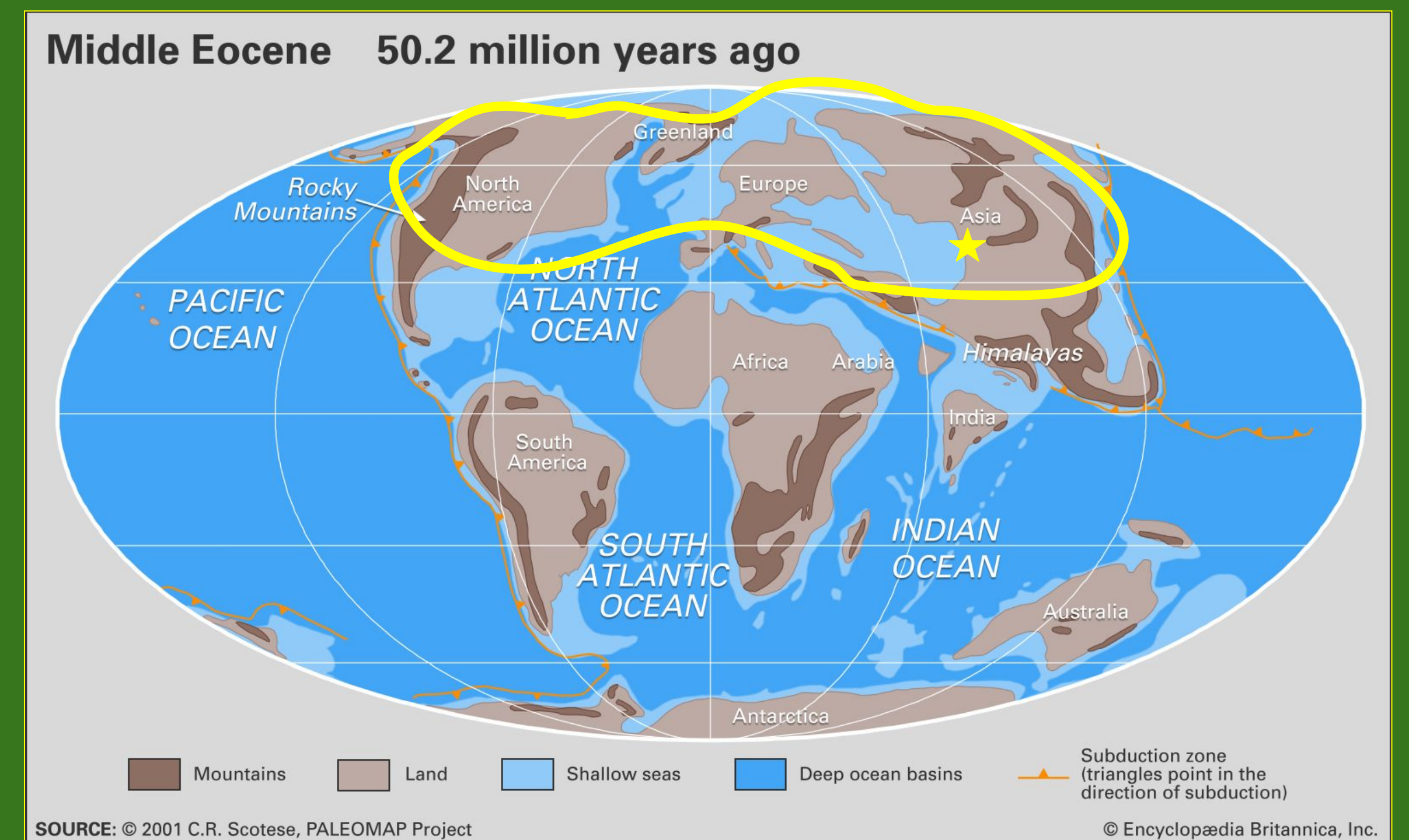
B. Map of the Middle Eocene with the Origin of Entelodont Starred and the Spread Circled
